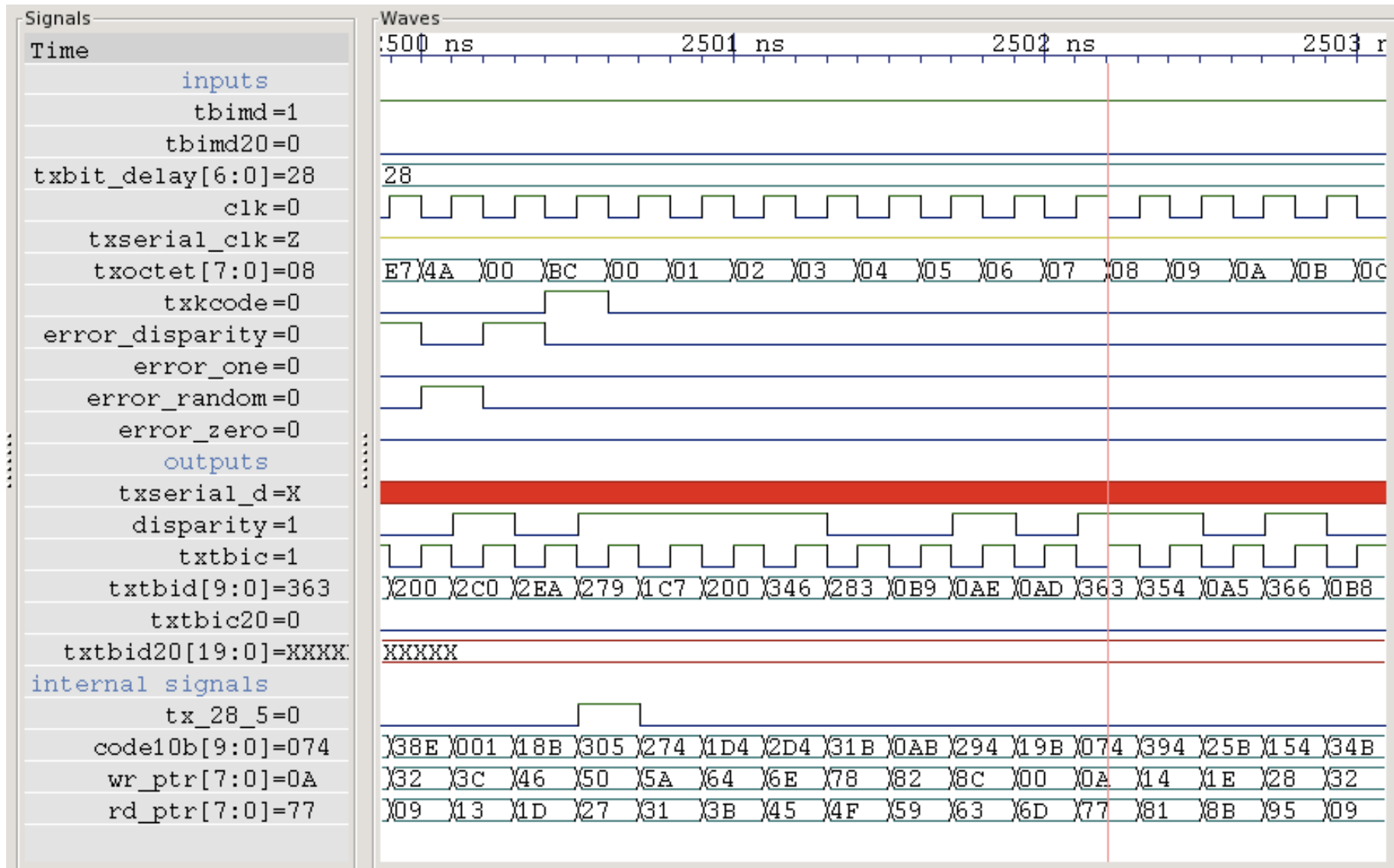
Figure A1.1 Timing Diagram of 8b10b encoder with 10 bit output enabled.
