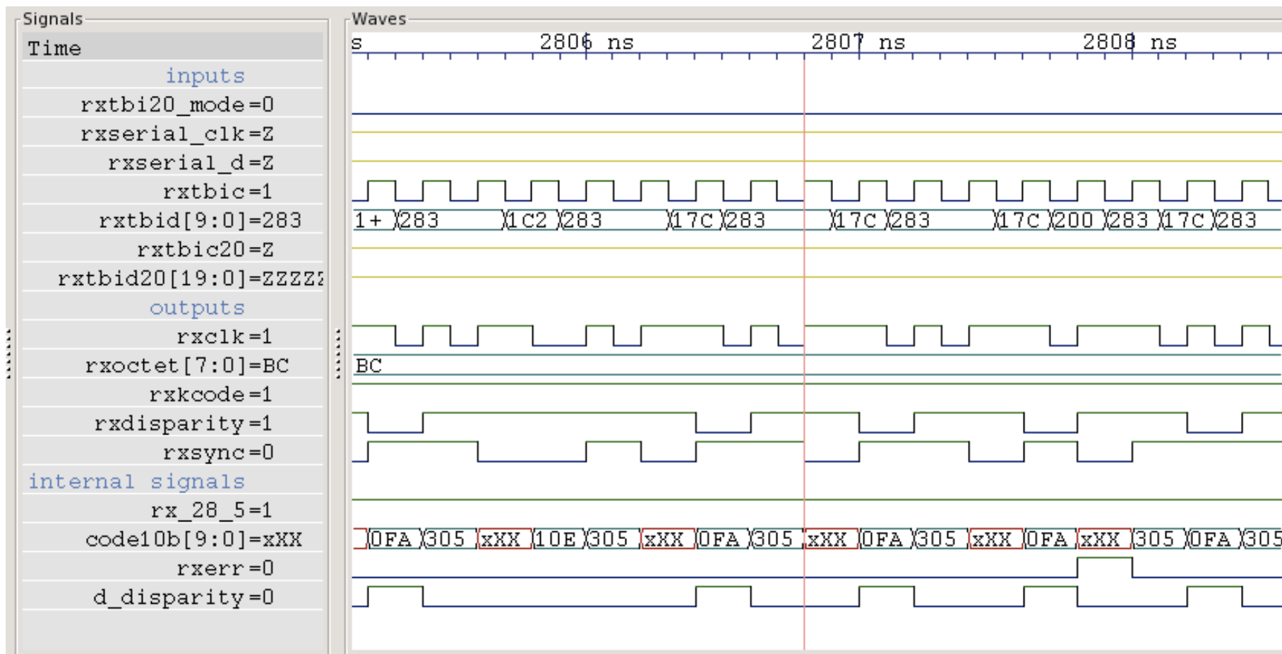
Figure A1.4 Timing Diagram of 8b10b decoder with 10 bit input active
